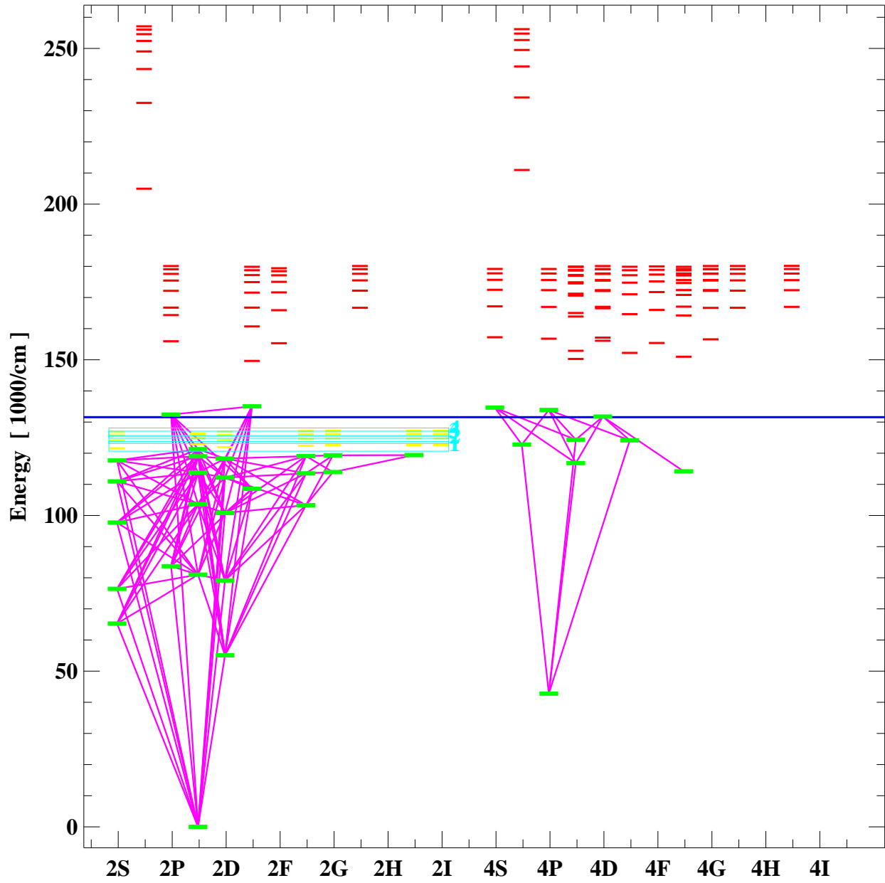
Grotrian diagram for si2
