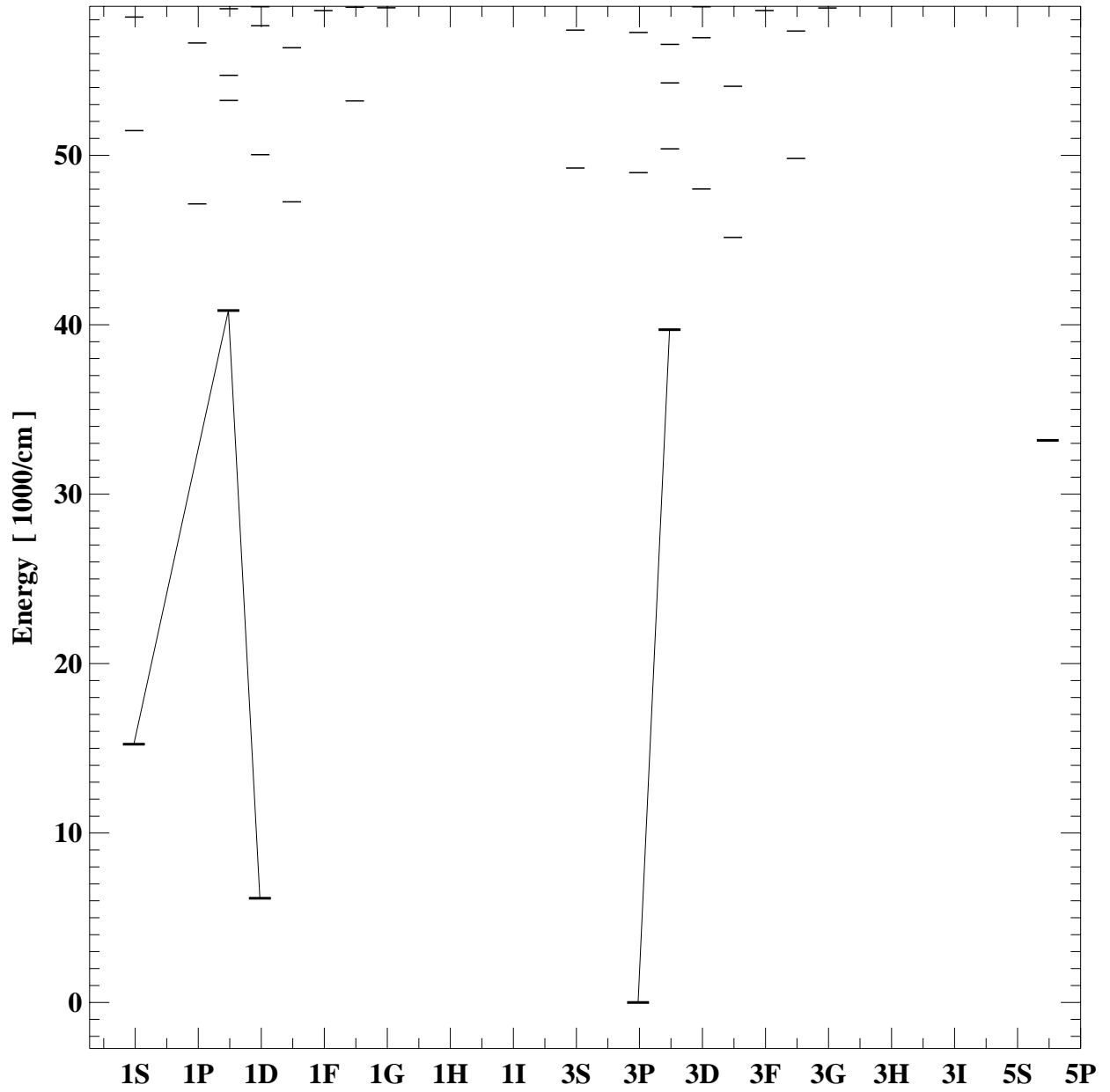
Grotrian diagram for Si1
