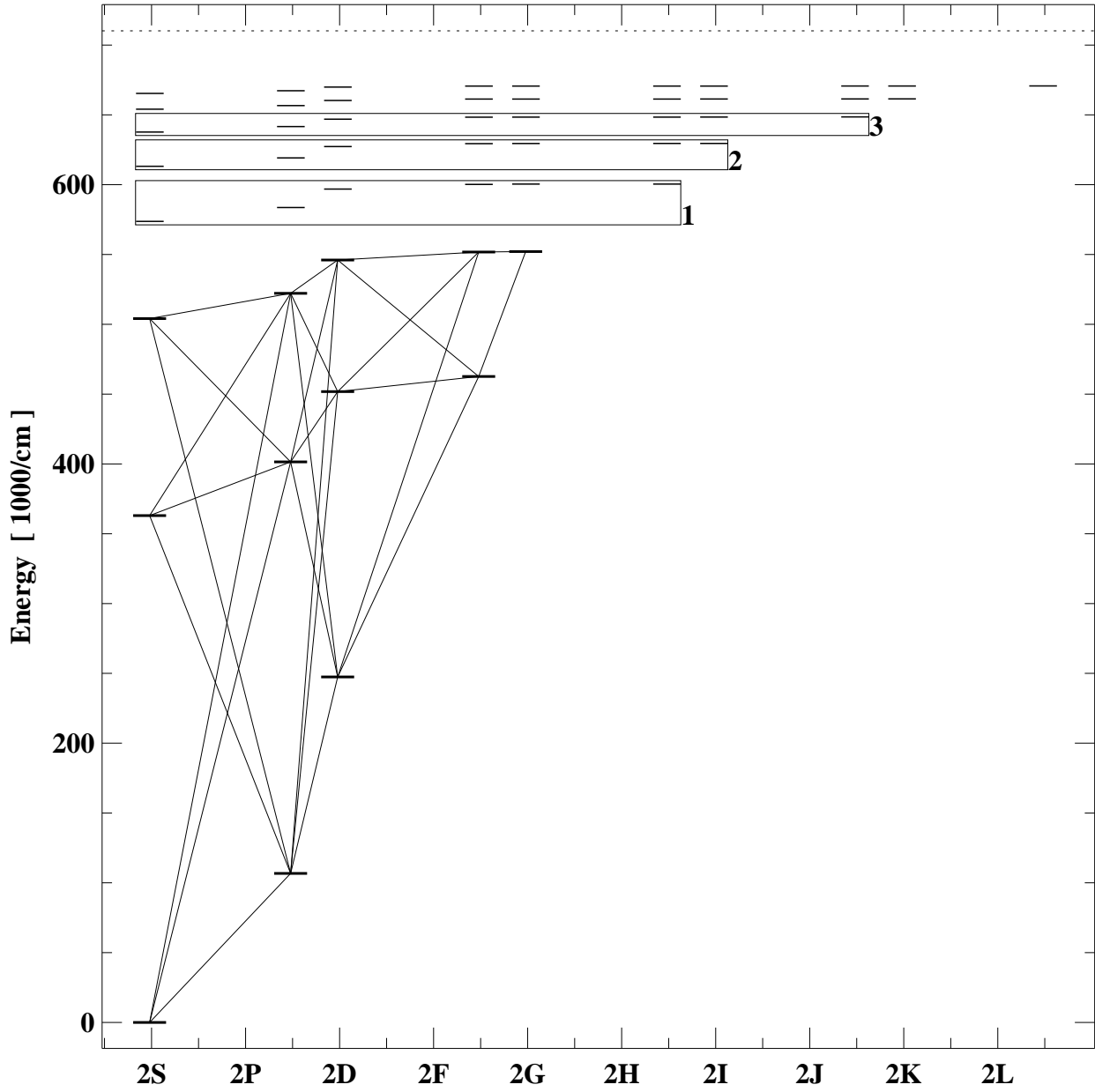
Grotrian diagram for s6
