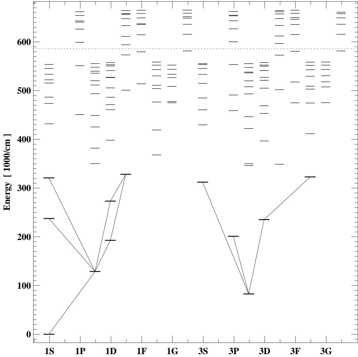
Grotrian diagram for s5
