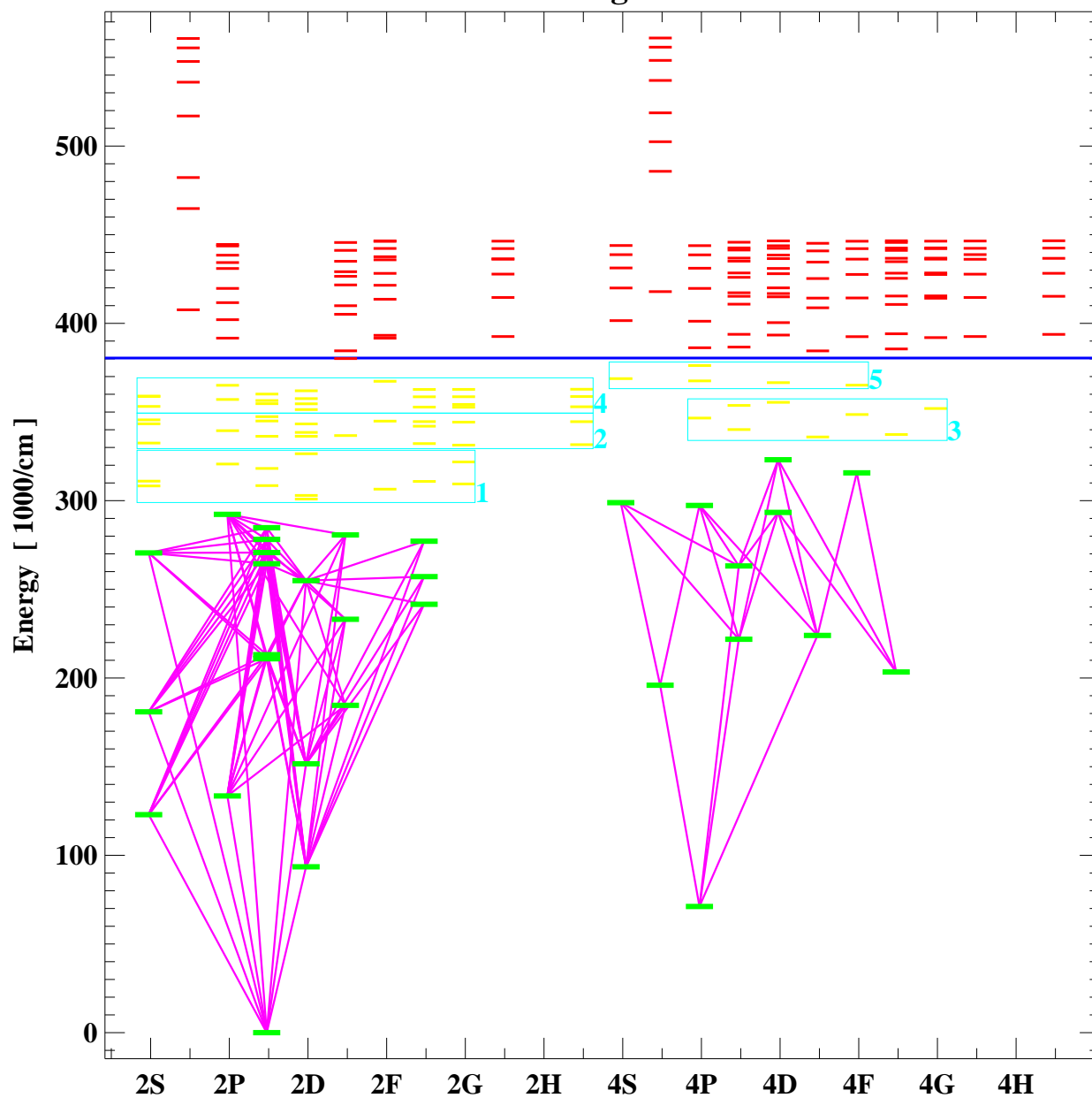
Grotrian diagram for s4
