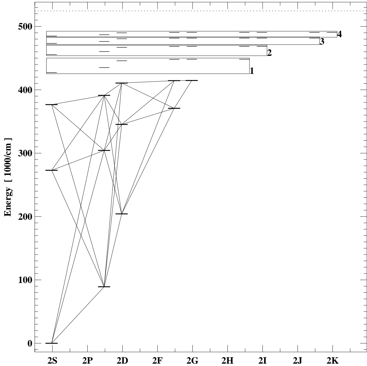
Grotrian diagram for p5
