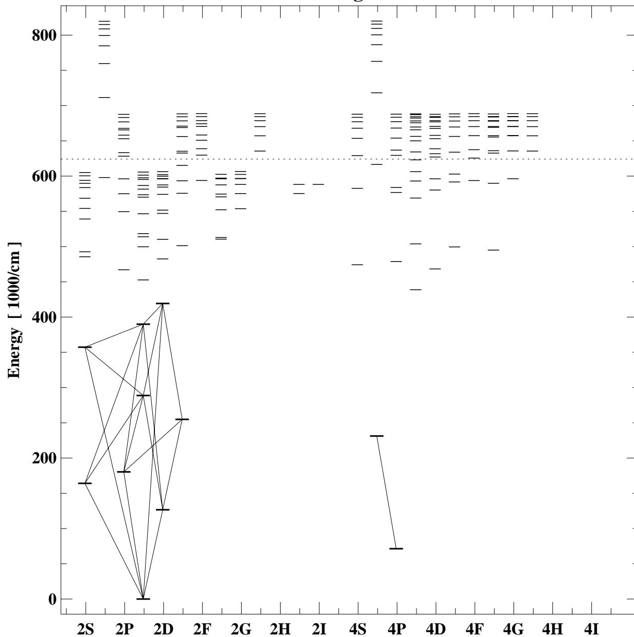
Grotrian diagram for o4
