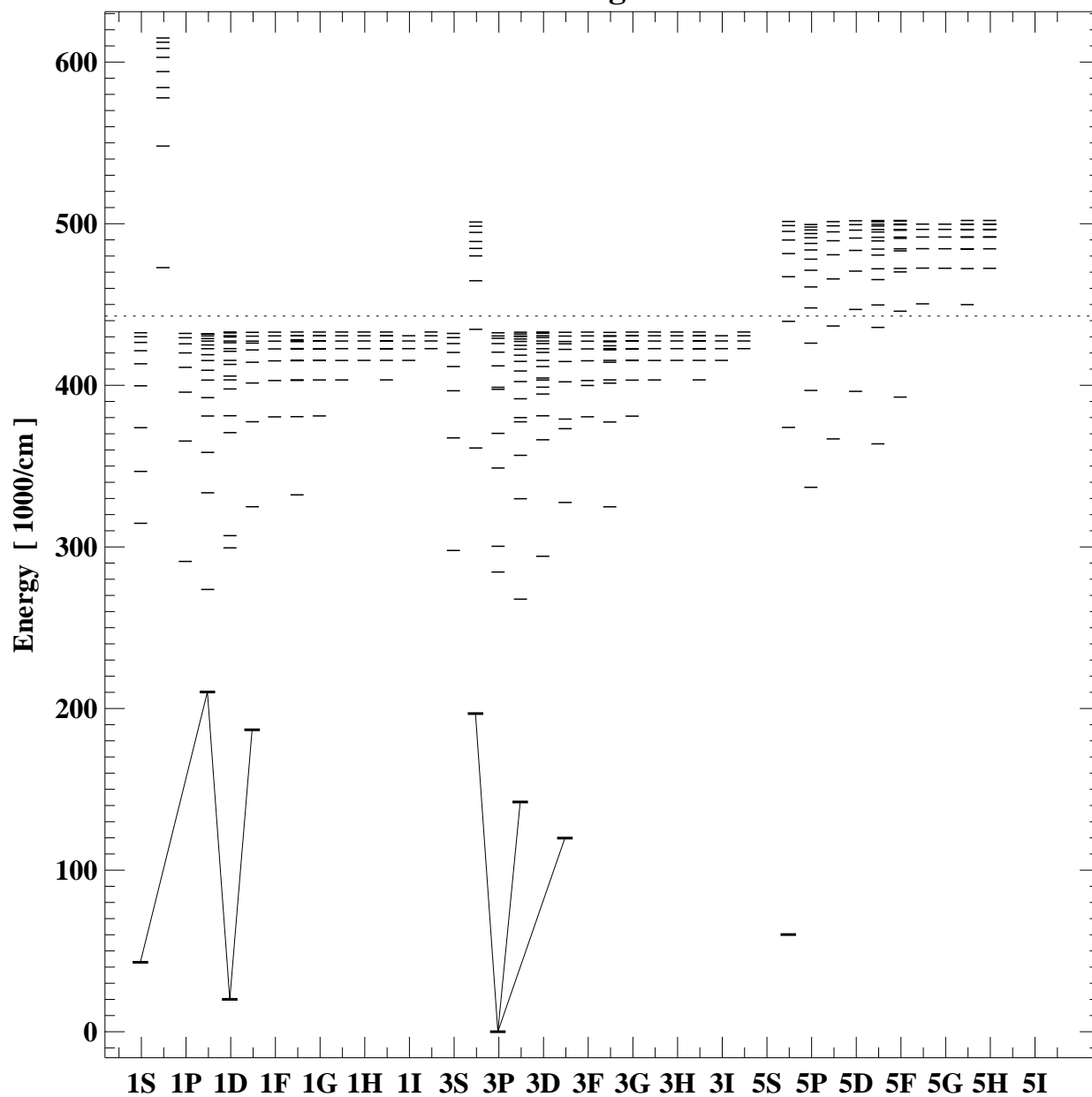
Grotrian diagram for o3
