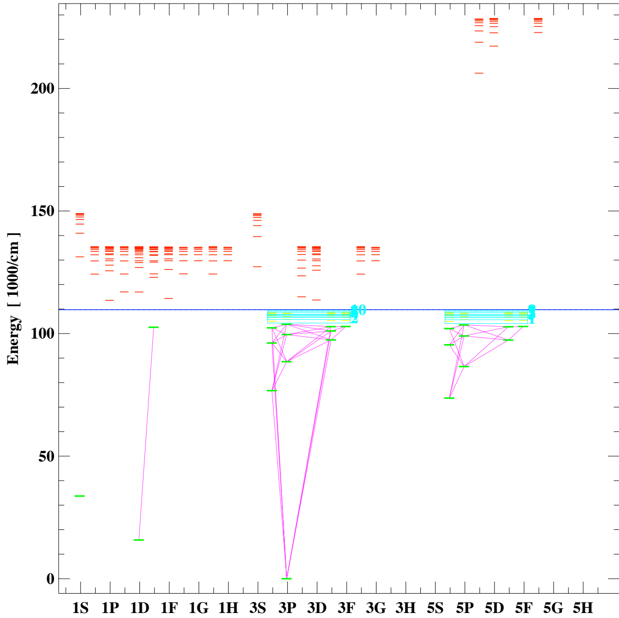
Grotrian diagram for o1
