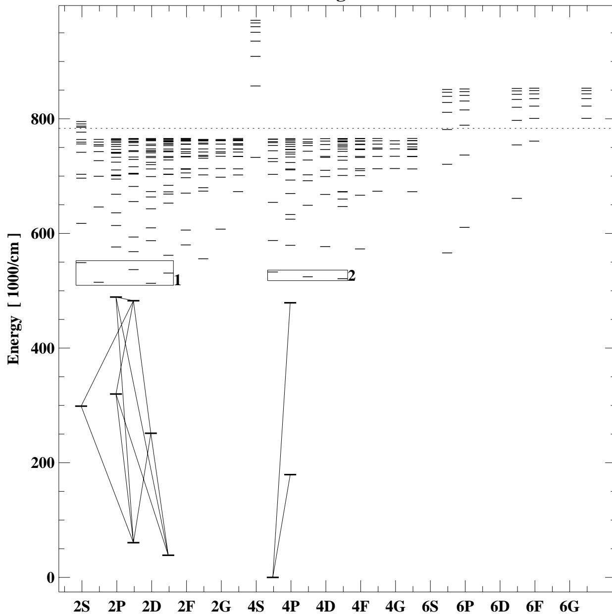
Grotrian diagram for ne4
