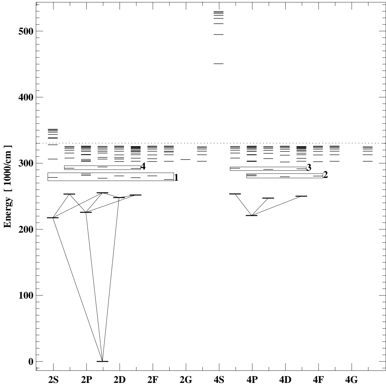
Grotrian diagram for ne2
