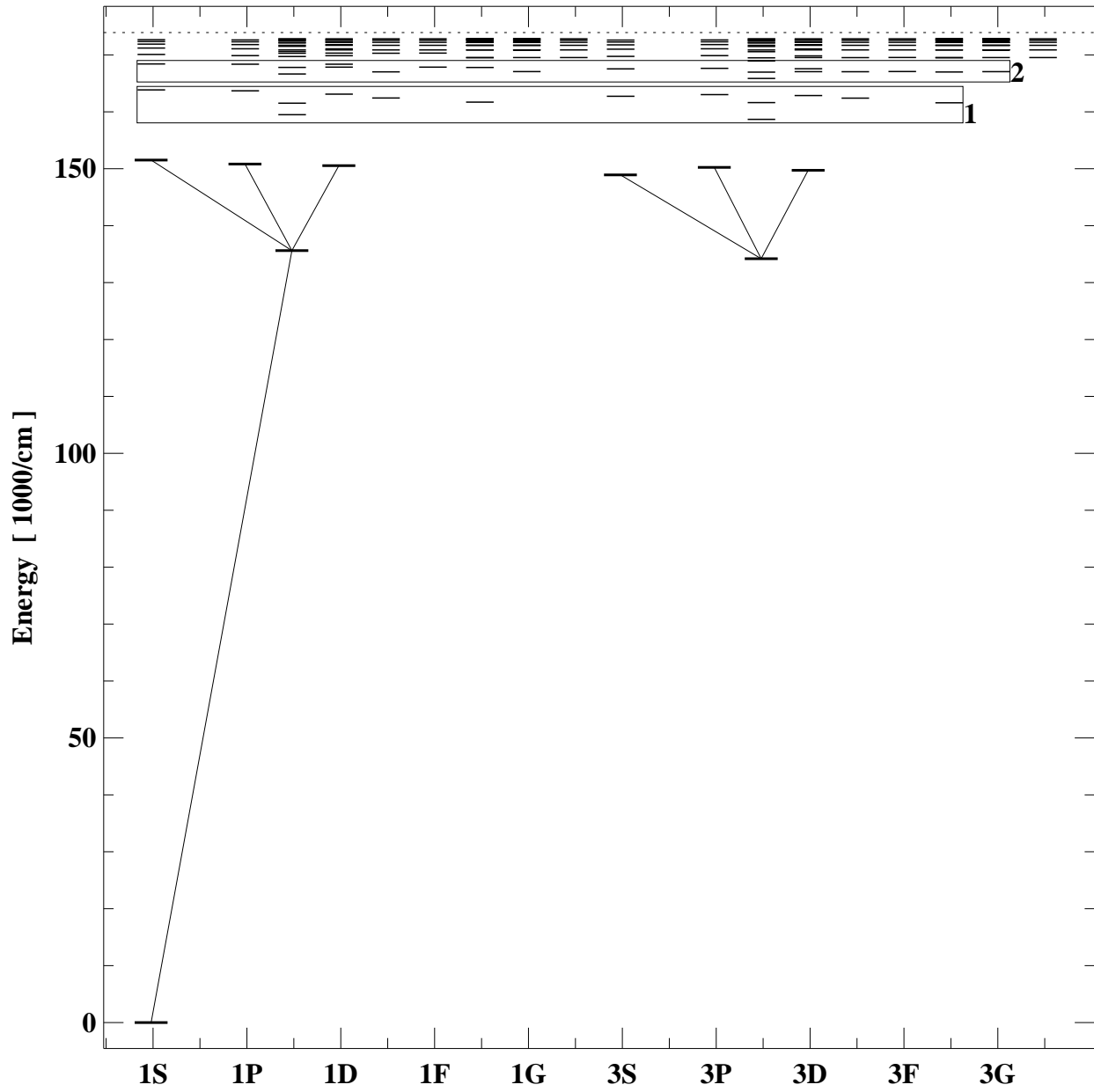
Grotrian diagram for ne1
