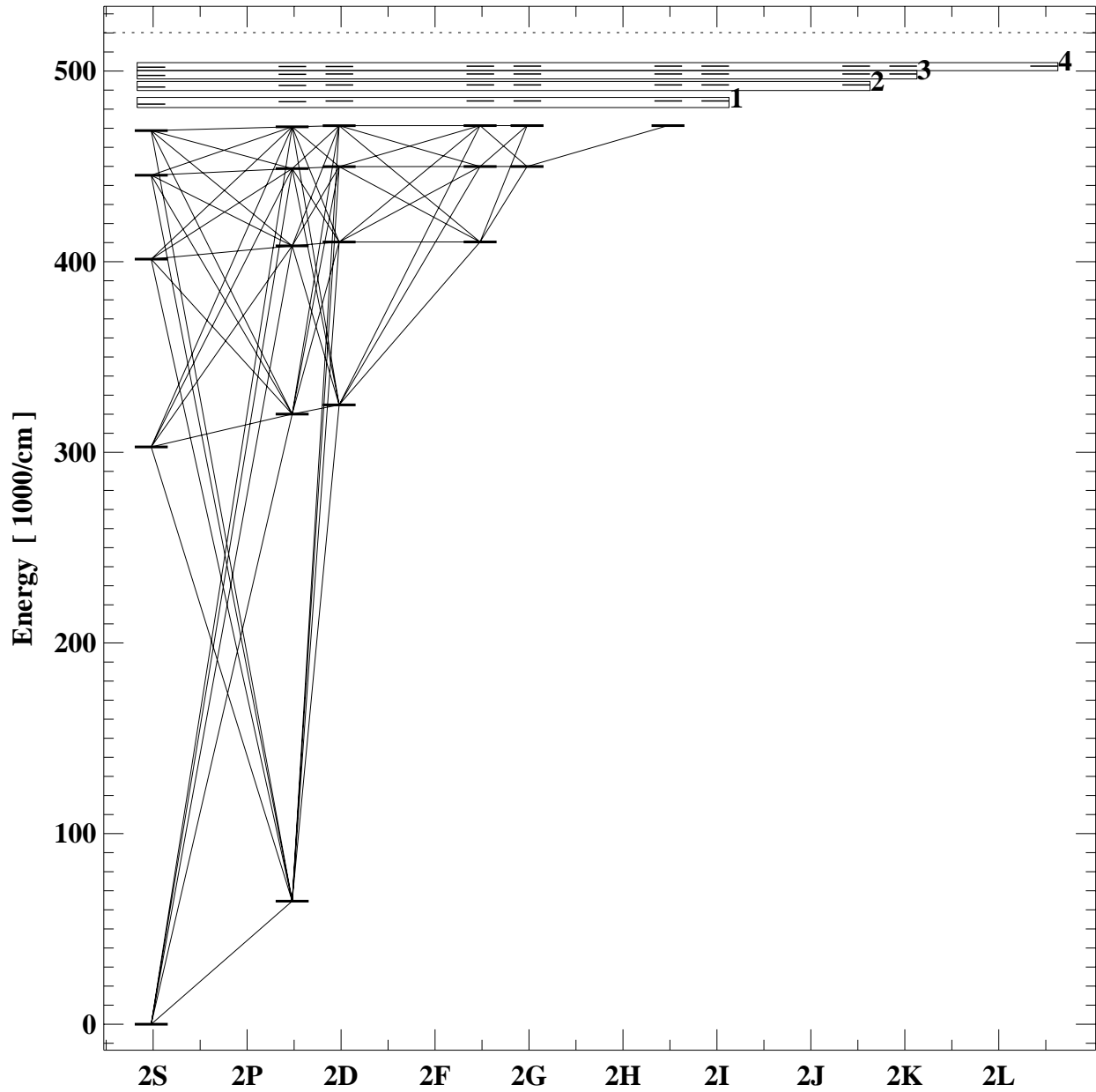
Grotrian diagram for c4
