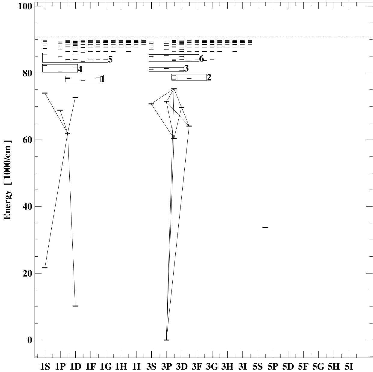
Grotrian diagram for c1
